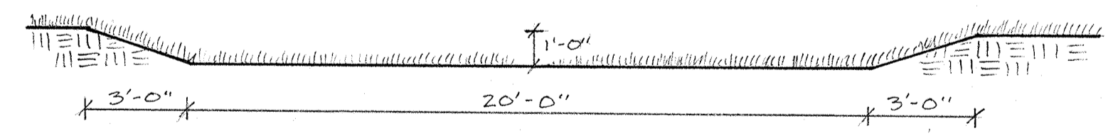
A I DETENTION BASIN CROSS SECTION SCALE 1/4" = 1'-0"
